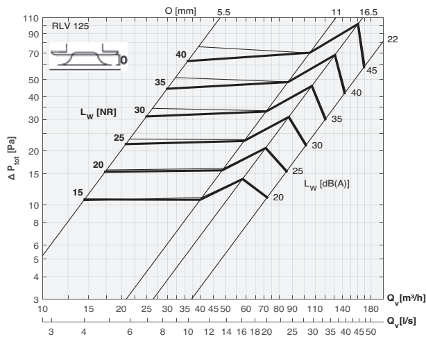
Pressure-volume flow characteristic curves for exhaust air
