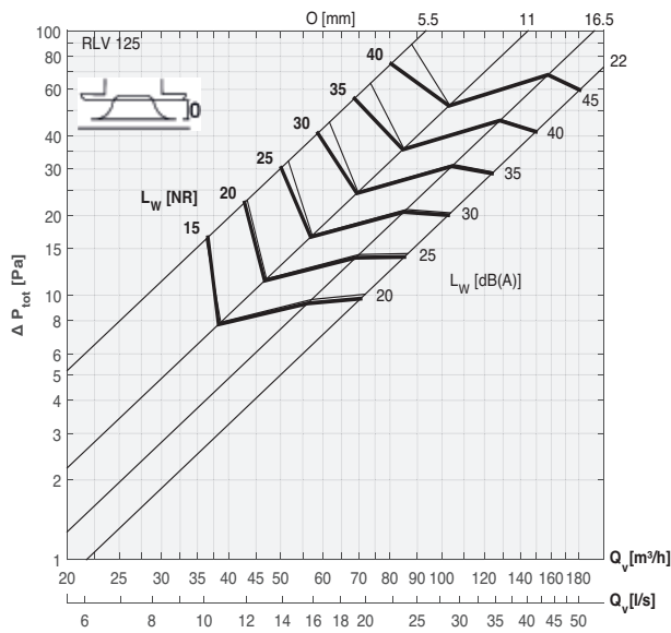
Pressure-volume flow characteristic curves for supply air
