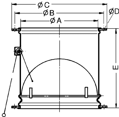
Dimensioned drawing [mm]
