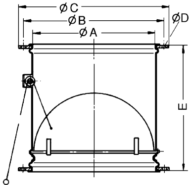
Dimensioned drawing [mm]
