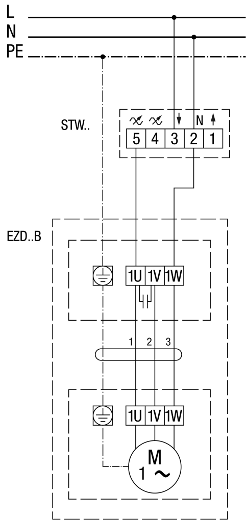
EZD ..B with STW speed controller
