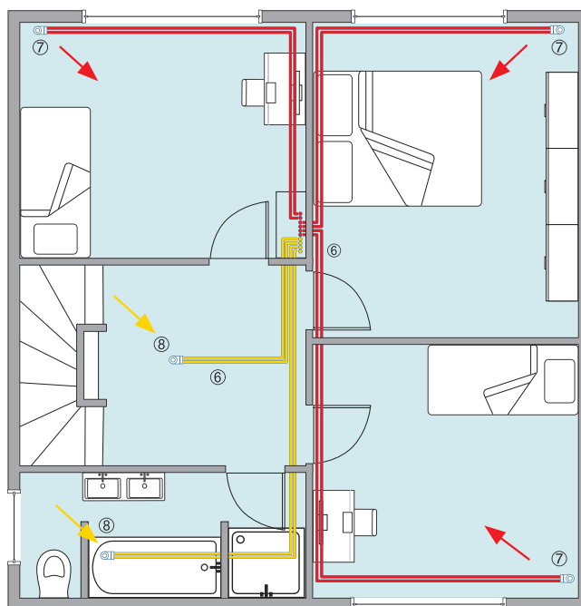
Upper floor
